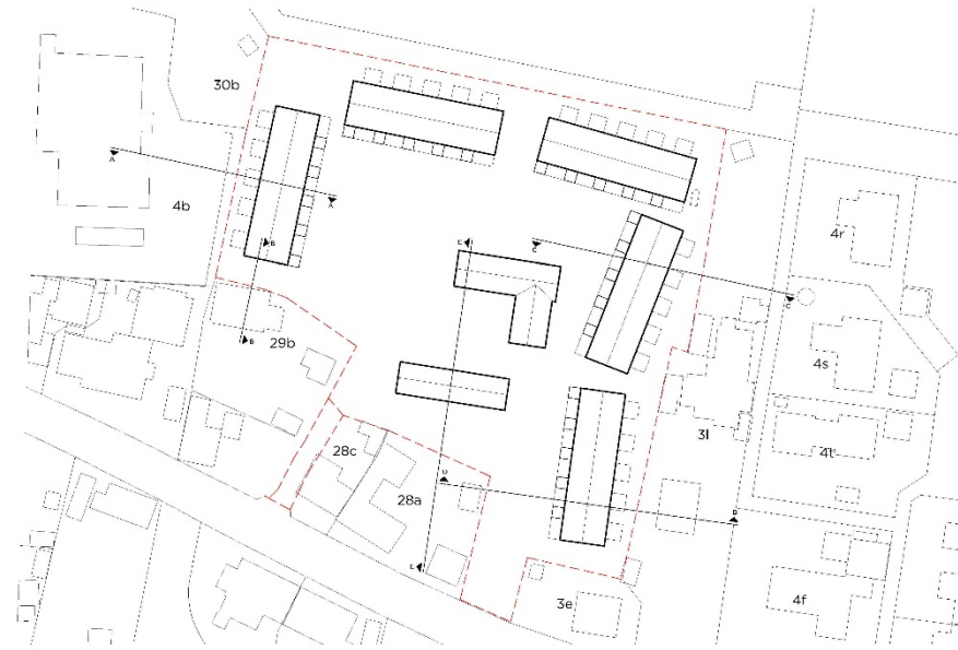
SITPLAN SNIT 1:500
